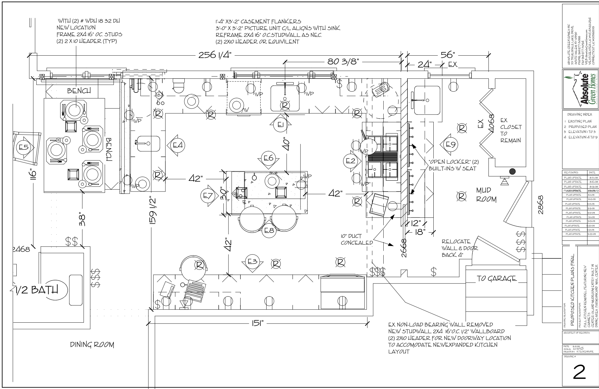
PROPOSED KITCHEN
