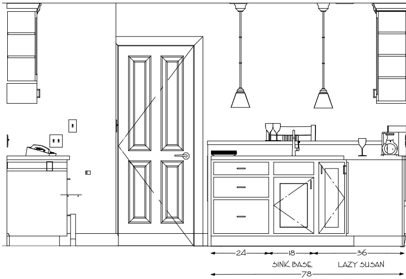
E4 PENINSULA
